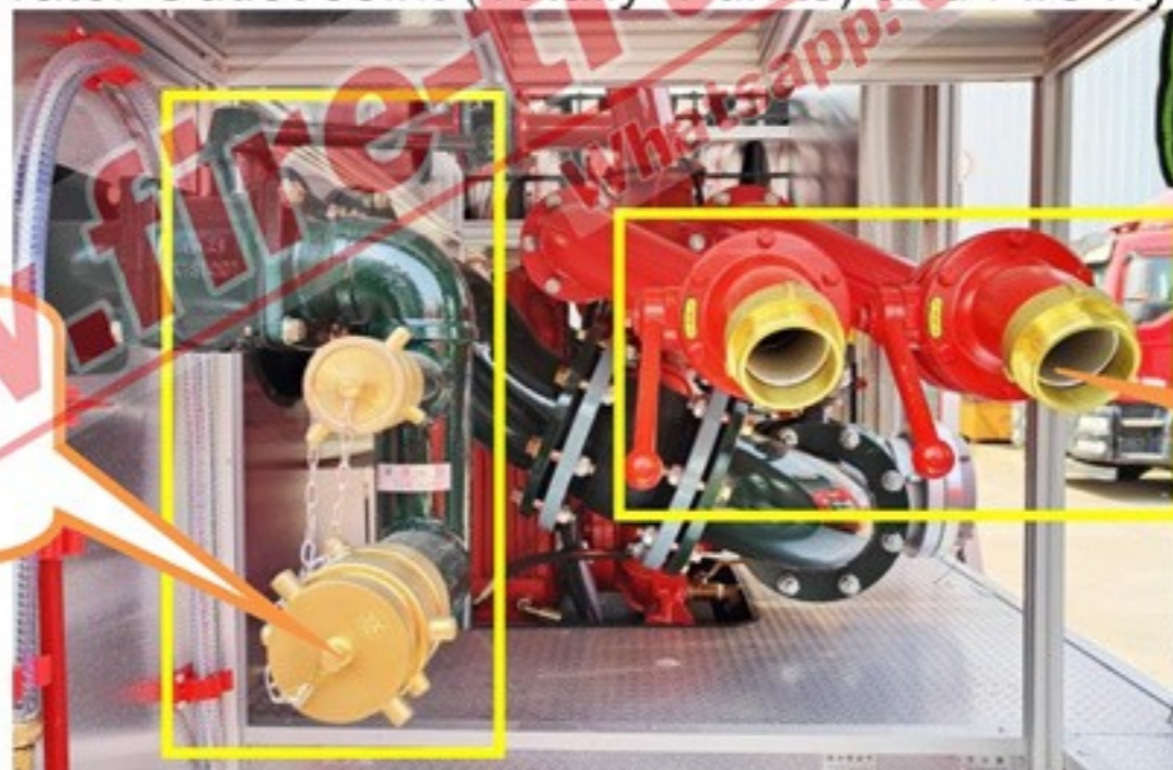
4 units Fire Hydrant Inlet Valve (each side has 2 units)
